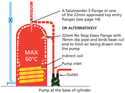
Figure 3: Hot water supply method
