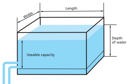
Figure 10: Water capacity calculations
