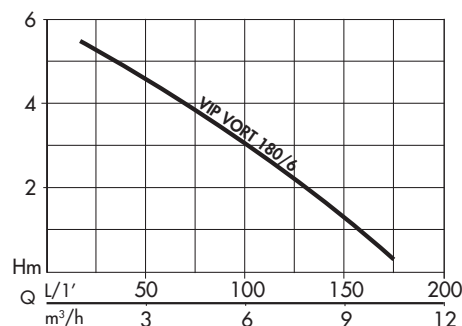
PERFORMANCE CURVE
